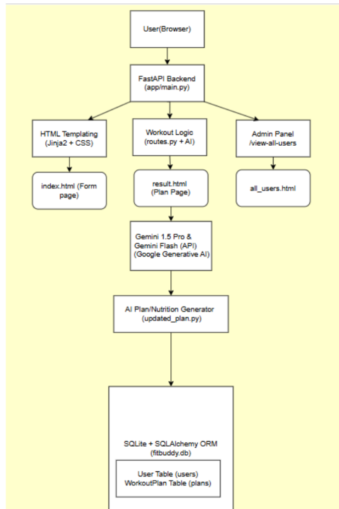
Figure: FitBuddy system architecture flow
