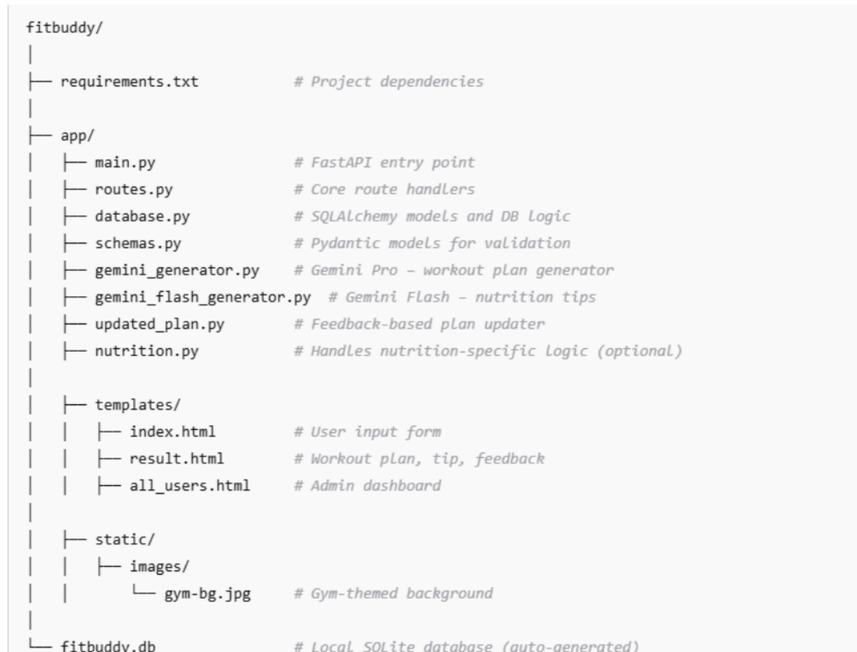
Figure: FitBuddy folder & file structure
